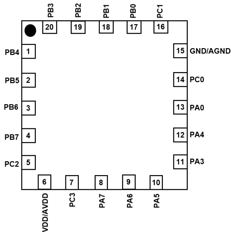
PFS123-1J20A: QFN3*3-20P
